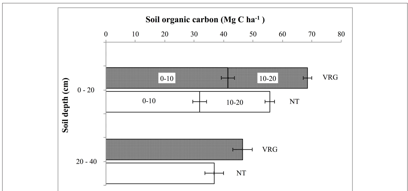
FIGURE 1 | Average ± SE of the distribution of organic carbon in the soil by depth for Voisin's Rational Grazing (VRG) pasture management and for fields with No-tillage crop system (NT) in Western Santa Catarina State, Brazil ( n = 5 ).
